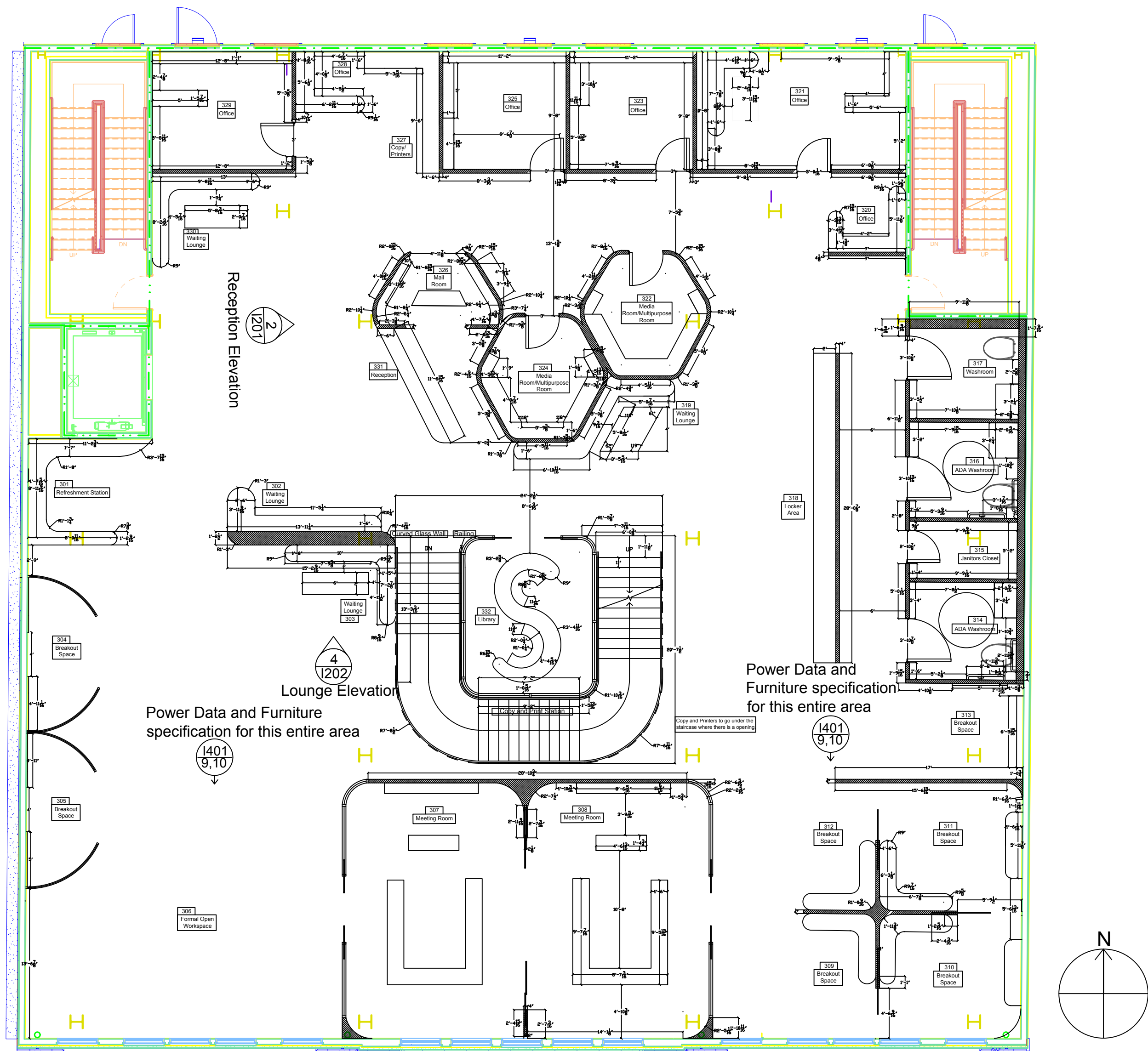
2. Third Floor Plan Scale: 1/8" = 1'-0"
