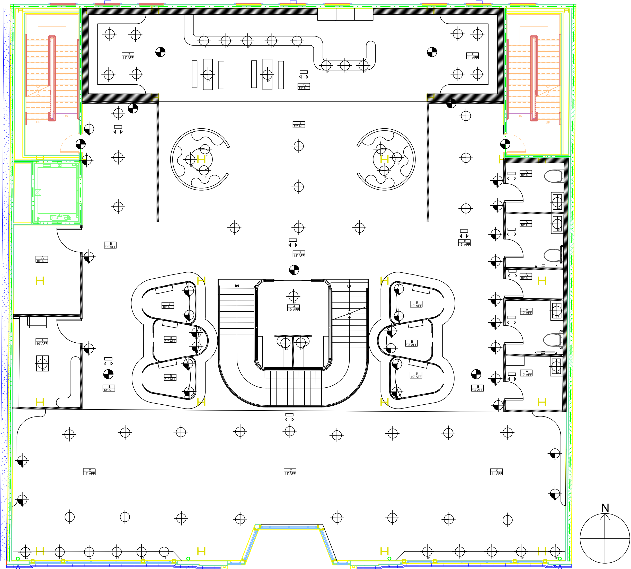
3. Second Floor Reflected ceiling plan
