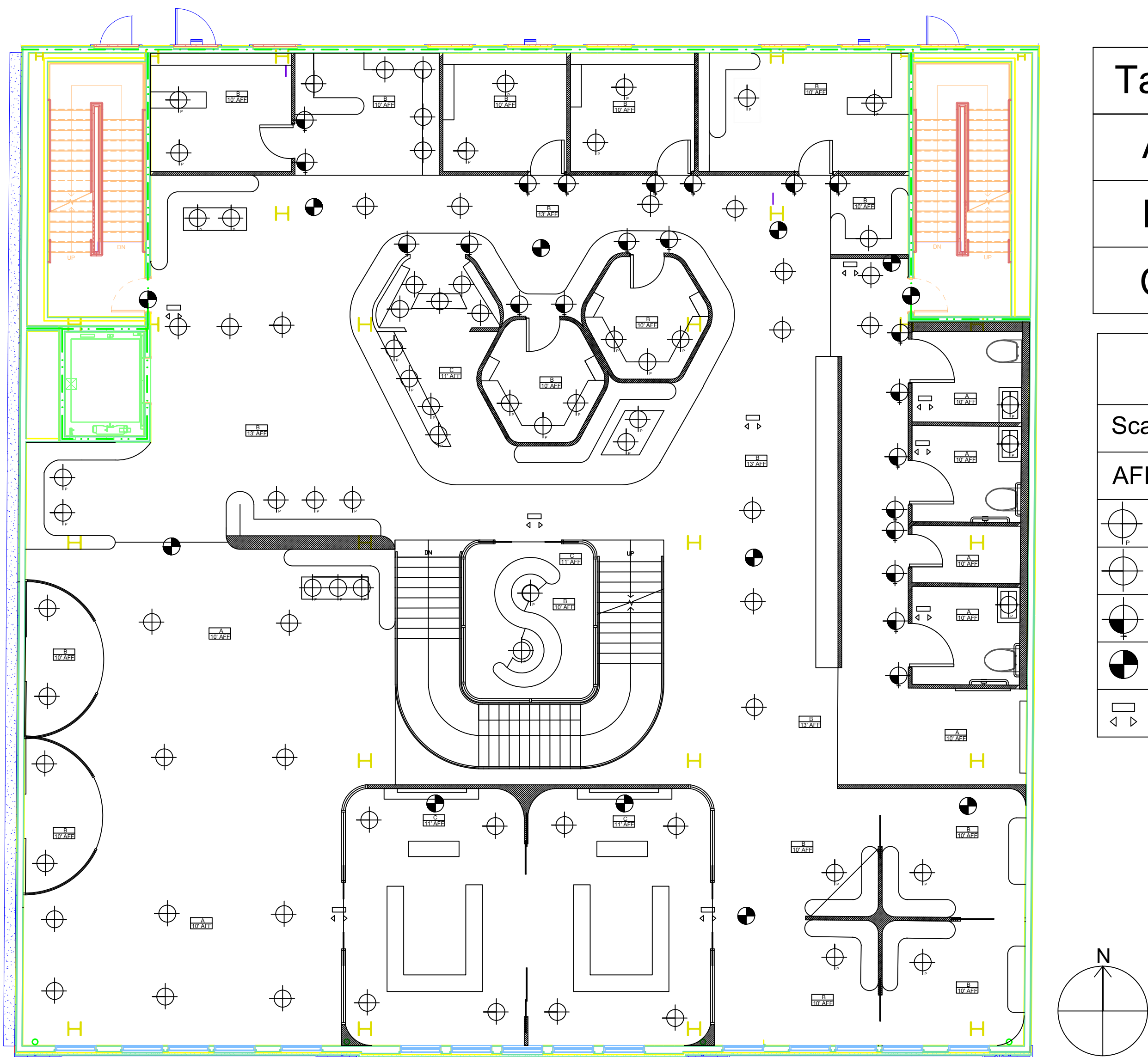
4. Third Floor Reflected ceiling plan Scale: 1/8" = 1'-0"
