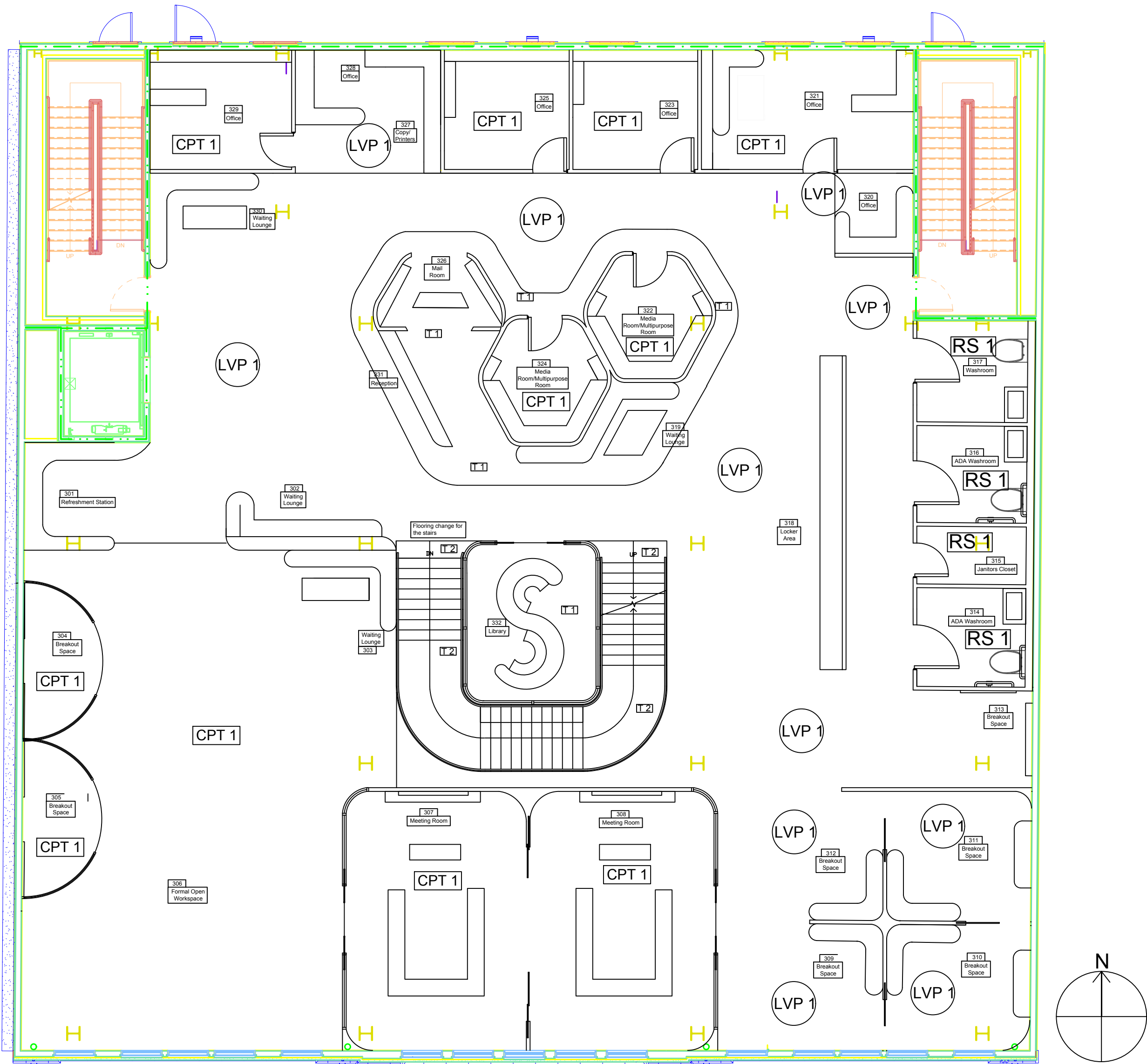
8. Third Floor- Floor Finish Plan Scale: 1/8" = 1'-0"
