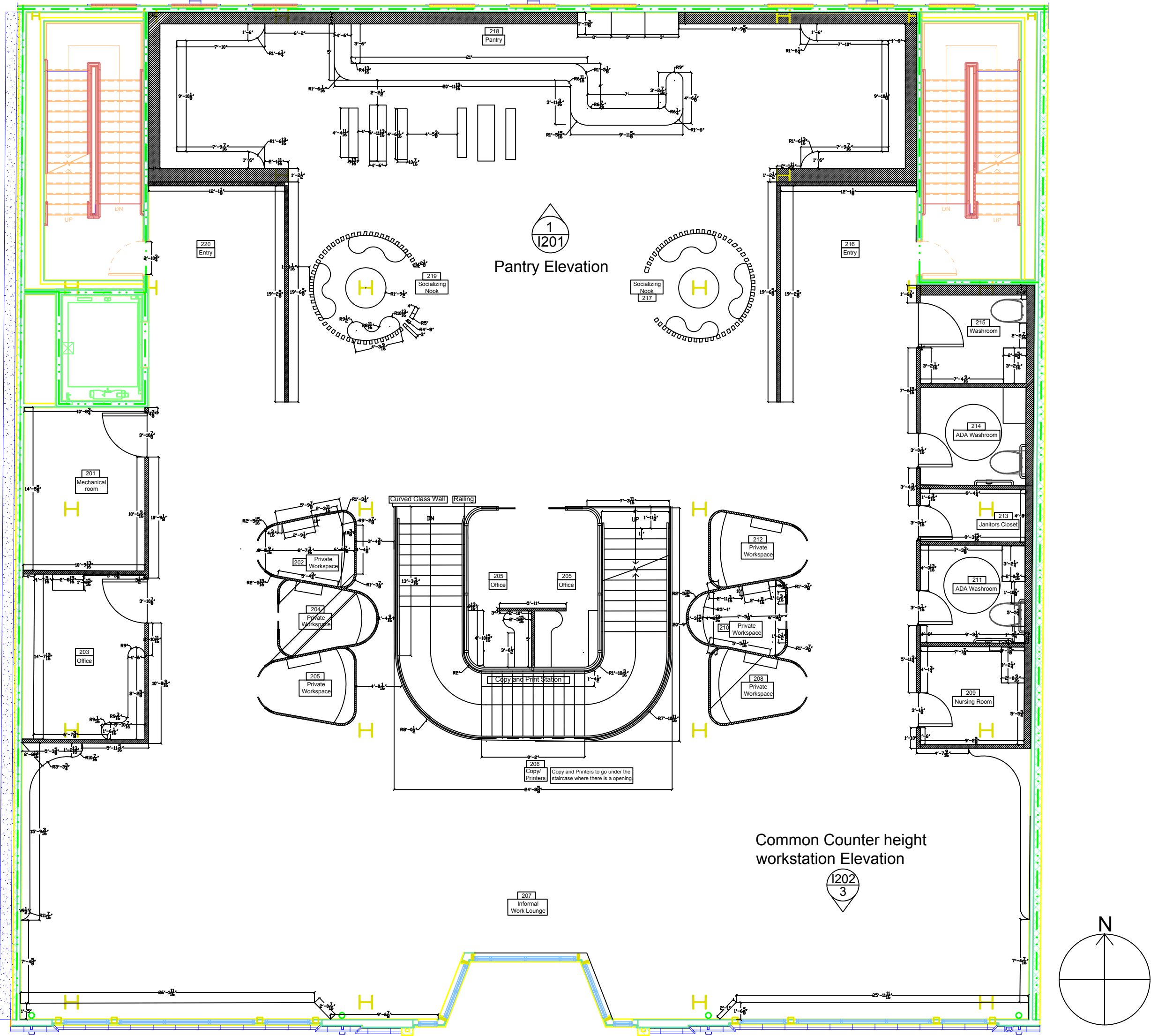
1. Second Floor Plan
