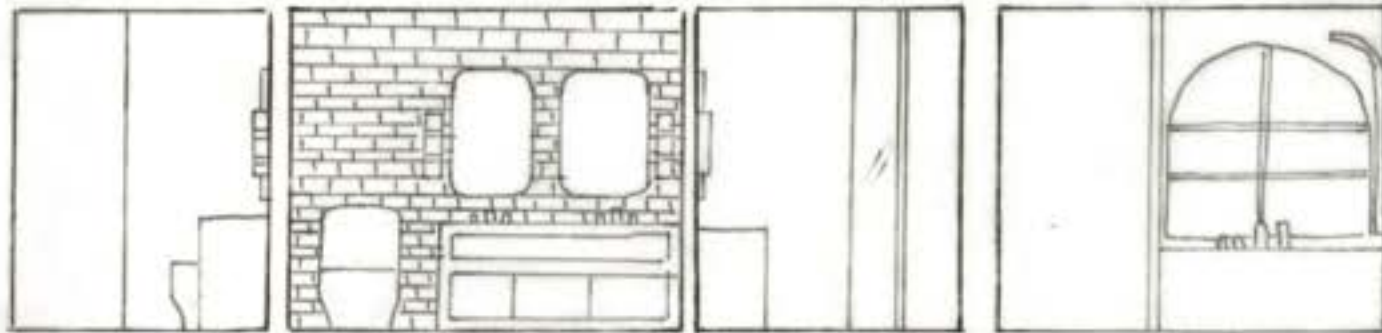
SOUTH ELEVATION
